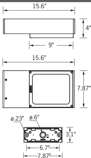
Mounting Detail
